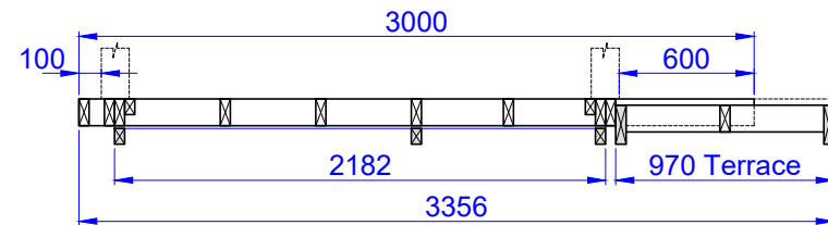
Cut view
