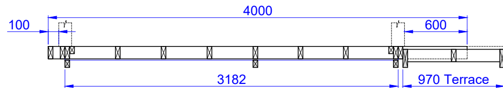
Cut view
